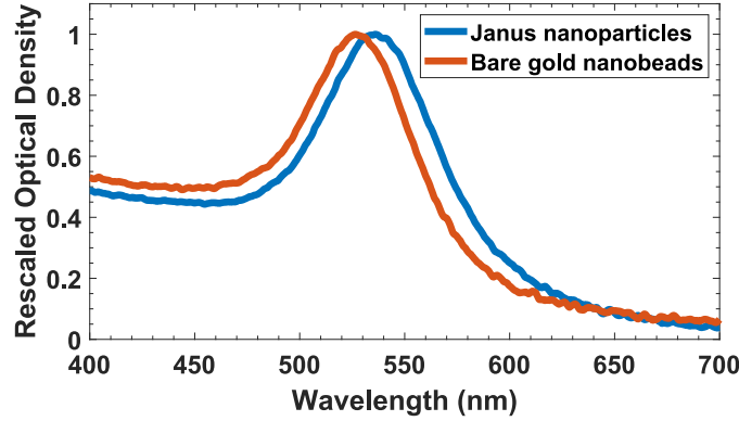
Figure 3: Visible absorption spectra of Janus nanoparticles (blue line) and bare gold nanobeads (orange line). For comparison purposes, the optical density of each spectrum has been normalized to its respective maximum absorption value to account for differences in sample concentration. The corresponding maximum optical densities are OD_{max,Au} = 3.56 and OD_{max,Janus} = 2.99 .
