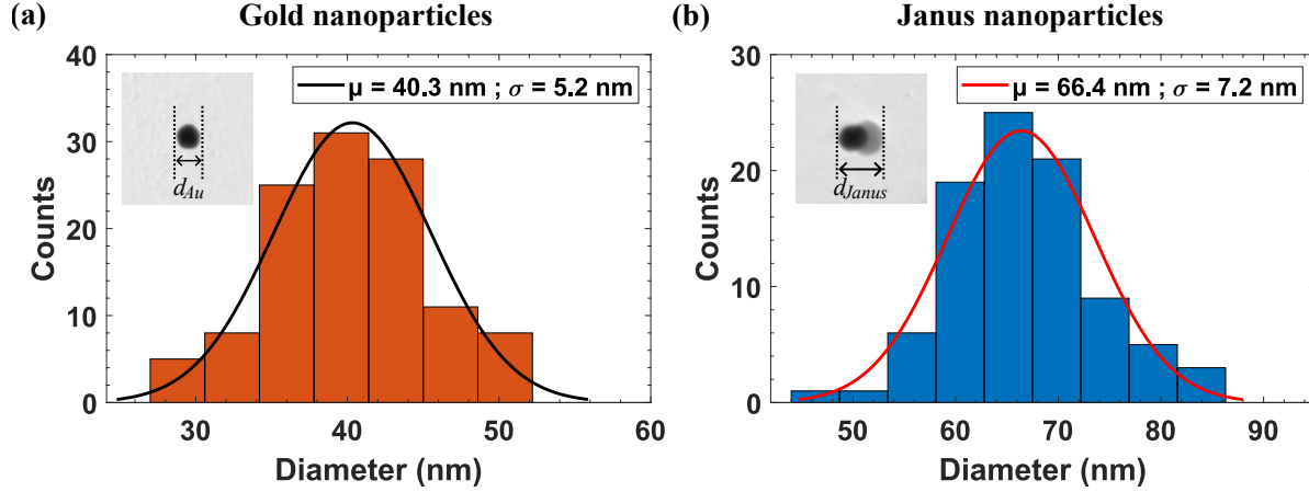
Figure 2: Nanoparticle size distribution determined by transmission electron microscopy (TEM). (a) Bare gold nanobeads ( N = 116 ) and (b) Janus nanoparticles ( N = 90 ). The gold nanobeads are nearly spherical, characterized by a diameter d_{Au} , while d_{Janus} refers to the major axis of the Janus nanoparticles (see inset). Solid lines represent Gaussian fits to the measured size distributions; error bars on the particle diameter correspond to the standard deviation of these fits: d_{Au} = 40.3 \pm 5.2 nm and d_{Janus} = 66.4 \pm 7.2 nm.
