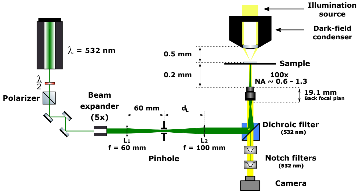
Figure 4: Schematic representation of the optical setup enabling both direct visualization of the sample via dark-field microscopy and its excitation using green laser illumination.
