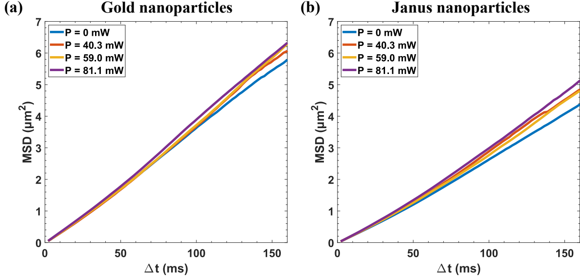
Figure 8: Ensemble-averaged mean squared displacements (MSDs) for (a) bare gold nanospheres and (b) Janus nanoparticles under increasing optical power. Data represent averages over about 100 individual particles (see Figures S1 and S2). In both systems, the increasing slopes of the MSD curves with higher illumination intensity indicate enhanced effective diffusion coefficients.
