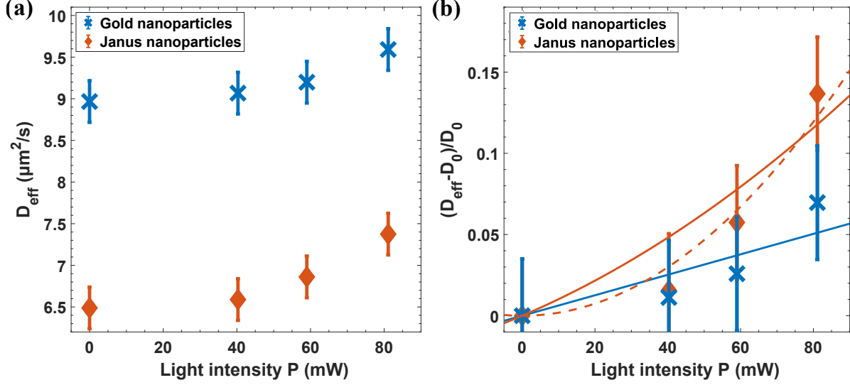
Figure 9: Experimental evidence of self-thermophoretic motion for Janus nanoparticles under optical illumination. (a) Effective diffusive coefficients extracted from MSD analysis increase with light intensity. The lower absolute diffusion values of Janus nanoparticles, compared to bare Au particles, stem from their larger size due to the silica shell. (b) Normalized effective diffusion coefficients as a function of laser intensity. D_0 is the diffusion coefficient in absence of illumination. The enhanced dynamics of Janus nanoparticles reveal light-activated self-propulsion in addition to hot Brownian motion, which is also observed for Au nanoparticles (linear fit (Eq. 5) shown as a blue line). Orange lines represent quadratic fits for Janus nanoparticles: the dashed curve is purely quadratic (Eq. 9, a = 0 ), while the solid curve includes the same linear contribution as for Au nanobeads (Eq. 9, a = 6.35 \times 10^{-4} , b = 9.85 \times 10^{-6} ). Error bars represent estimated experimental uncertainties.
