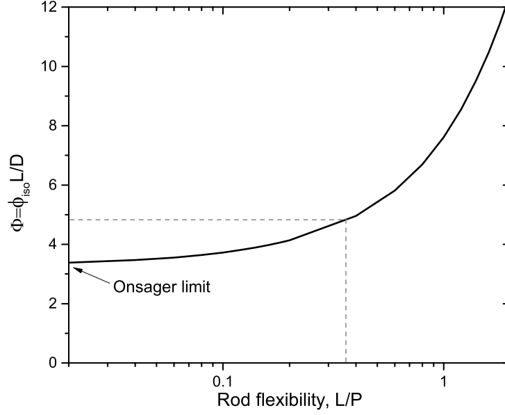
FIG. 2. Dimensionless concentration \Phi as a function of the rod flexibility L/P as predicted by Chen [2]. The dashed lines indicate the case of rod-like viruses studied in this work for which L/P = 0.36 and \Phi = 4.8 .
