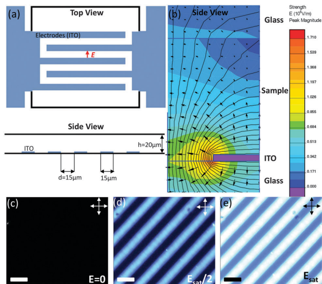
Fig. 2 (a) Schematic representation of the In-Plane Switching (IPS) cells used for probing the electro-optical effects in our colloidal dispersions. (b) Equipotential lines of the electric field ( f = 100 kHz) simulated by finite element method inside an IPS cell containing ethylene glycol. For symmetry reason, only half an electrode is represented (side view). (c) Observation by optical microscopy between crossed polarizers of an IPS cell (top view) filled with an isotropic liquid suspension of \text{LaPO}_4 nanorods when no electric field is applied (off-state). (d) and (e) Progressive increase of the electric induced birefringence with the in-plane electric field (scale bars: 30 \mu\text{m} ).
