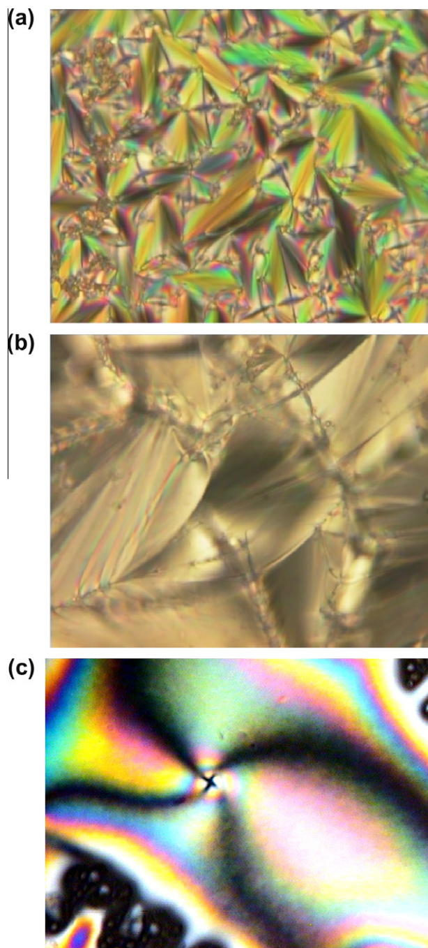
Fig. 2. The representative photomicrographs of (a) the focal conic texture of the SmA phase for compound 6c at 120 °C, (b) the SmA polygonal texture for compound 6d at 160 °C and (c) the nematic schlieren texture for compound 7c at 241 °C (240 × 300 μm 2 ).
