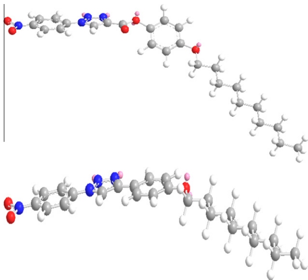
Fig. 3. Energy minimized structures of compound 6a (top) and homologous structure without ester function connector (bottom).
