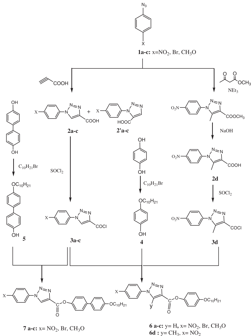
Scheme 1. Synthesis of compounds.
