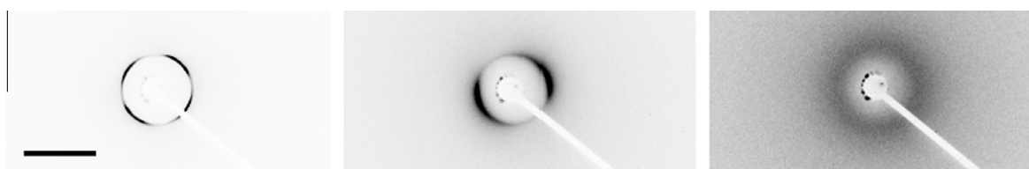
Fig. 5. X-ray diffraction pattern of the smectic (left), nematic (middle), and isotropic liquid (right) of the BiPhMeO, recorded at T = 170, 235 and 245 °C, respectively. The scale bar indicates 3 \text{ nm}^{-1} .
