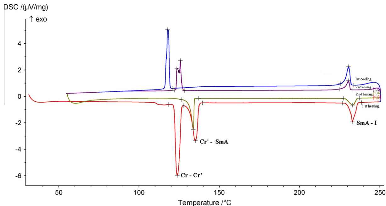
Fig. 4. Thermogram of compound 6a obtained by DSC during the first cycle at 10 °C/mn and during the second cycle at 5 °C/mn.
