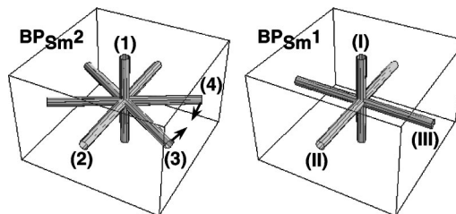
FIG. 1. Geometrical figures indicating the directions where the smectic order is enhanced, corresponding to the “Bragg peaks,” for the BP Sm 2 and cubic BP Sm(A) 1 monodomains probed by x-ray scattering. The arrows show their evolution during the transition between the two smectic blue phases (from Ref. [8]).
