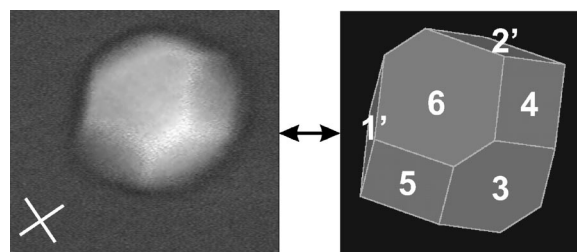
FIG. 5. Faceted monodomain of the \text{BP}_{\text{Sm}2} phase exhibiting four large and two small facets, as schematically shown in the corresponding pictures.
