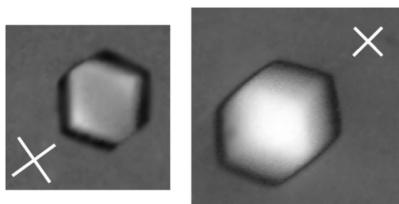
FIG. 3. Two other examples of the \text{BP}_{\text{Sm}2} monodomains observed along a twofold axis. An apex angle of about 110^\circ can also be found as in Fig. 2.
