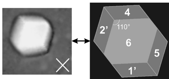
FIG. 2. Experimental and schematic view of a \text{BP}_{\text{Sm}2} monocrystal floating in the supercooled \text{BP}_{\text{Sm}3} and observed along a twofold axis in transmission between crossed polarizers. The white cross represents the projection (or the normal direction) of the optical axis in the observation plane.
